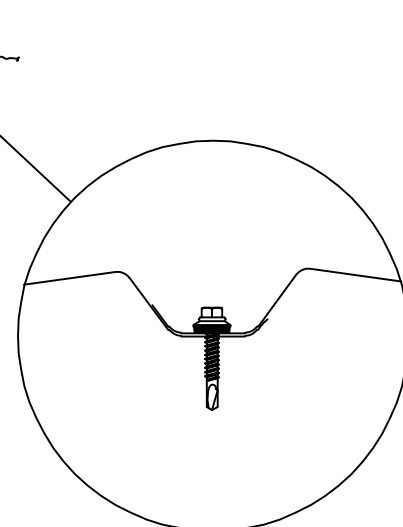
PANEL SIDE LAP
