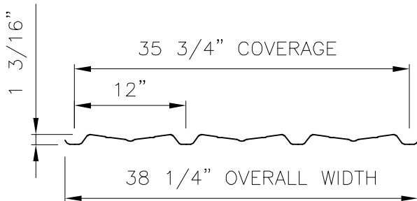
MULTI-V PANEL PROFILE
